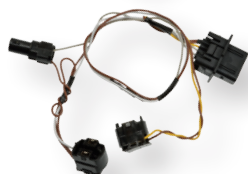
HWH700 Headlight Wiring Harness Mercedes E-Class 2000-96 VIO over 150,000
