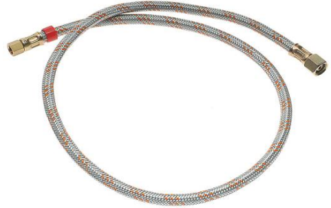
Red Hose Overall Length 41" 1/8" Female NPT x 14mm Female
