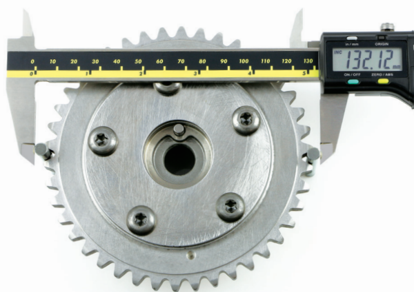
Sprocket Over Pin Diameter comparison
